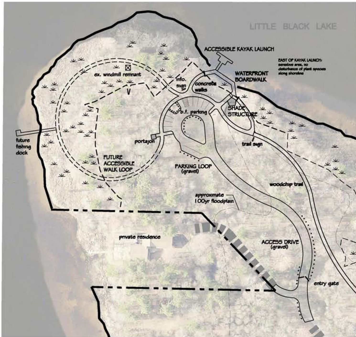
Little Black Lake Park Entrance Enlargement Plan
